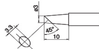
T17-BCF3 Shape-3BC *Tinned cut surface only B2900 Nozzle assembly G
