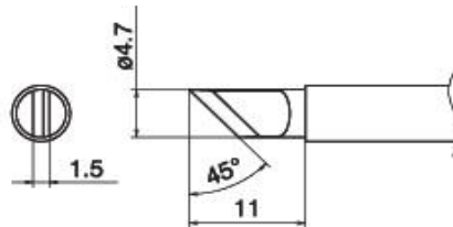
T17-KR Shape-KR B2902 Nozzle assembly I
