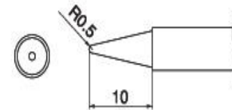
T17-B2 Shape-0.5B B2708 Nozzle assembly C
