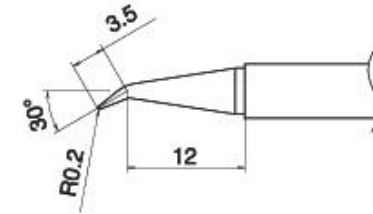
T17-J02 Shape-0.2J B2707 Nozzle assembly B
