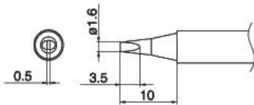
T17-D16 Shape-1.6D B2708 Nozzle assembly C
