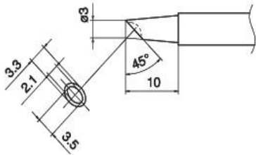
T17-BCM3 Shape-3BC Bevel with indent B2900 Nozzle assembly G
