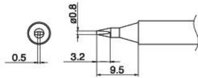
T17-D08 Shape-0.8D B2709 Nozzle assembly D
