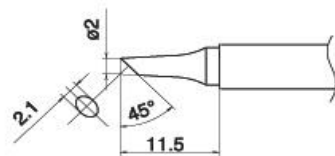
T17-BCF2 Shape-2BC *Tinned cut surface only B2706 Nozzle assembly A
