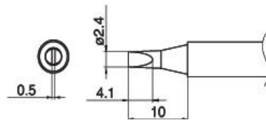
T17-D24 Shape-2.4D B2708 Nozzle assembly C
