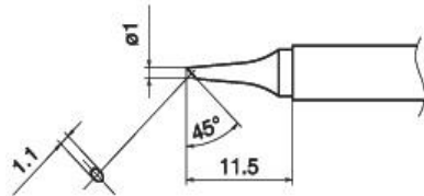
T17-BCF1 Shape-1BC *Tinned cut surface only
