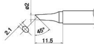
T17-BC2 Shape-2BC B2706 Nozzle assembly A
