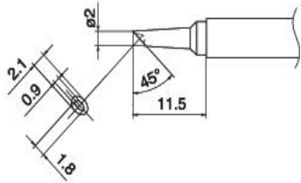
T17-BCM2 Shape-2BC Bevel with indent B2706 Nozzle assembly A
