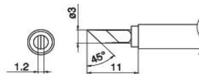
T17-KU Shape-KU B2901 Nozzle assembly H
