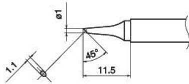
T17-BC1 Shape-1BC B2899 Nozzle assembly F
