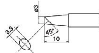
T17-BC3 Shape-3BC B2900 Nozzle assembly G
