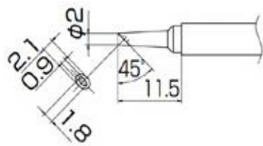
T13-BCM2 Shape-2BC Bevel with indent B2706 Nozzle assembly A
