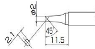
T13-BC2 Shape-2BC B2706 Nozzle assembly A
