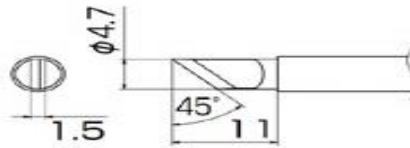
T13-KR Shape-KR B2902 Nozzle assembly I
