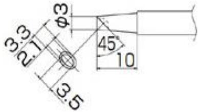
T13-BCM2 Shape-2BC Bevel with indent B2706 Nozzle assembly A
