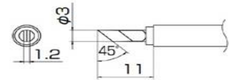
T13-KU Shape-KU B2901 Nozzle assembly H
