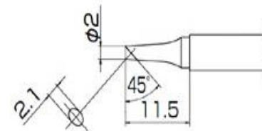
T13-BCF2 Shape-2BC Tinned cut surface only B2706 Nozzle assembly A
