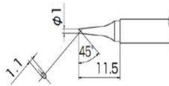
T13-BCF1 Shape-1BC Tinned cut surface only B2899 Nozzle assembly
