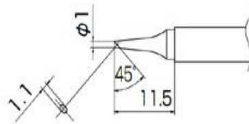
T13-BC1 Shape-1BC B2899 Nozzle assembly F
