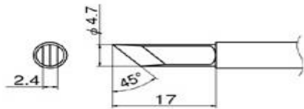
T13-KF Shape-KF B2923 Nozzle assembly J
