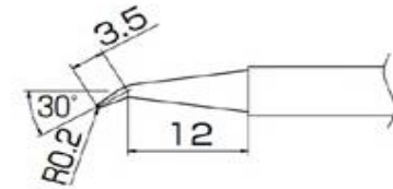
T13-J02 Shape-0.2J B2707 Nozzle assembly B
